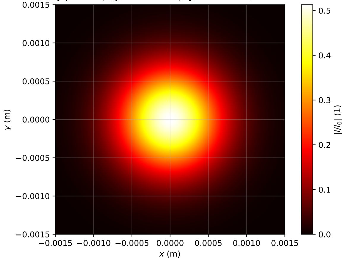
Intensity profile I(x, y, z = 2.309m)/I_0 , P_{in}=0.2P_{cr} , artificial time
